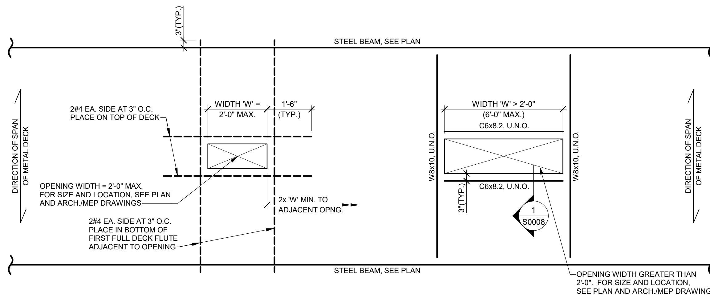
SLAB REINFORCED CONDITION (2'-0" MAX. OPENING WIDTH)
