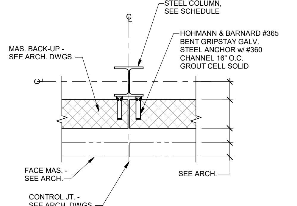
TYPICAL MASONRY CONTROL JOINT AT COLUMN
