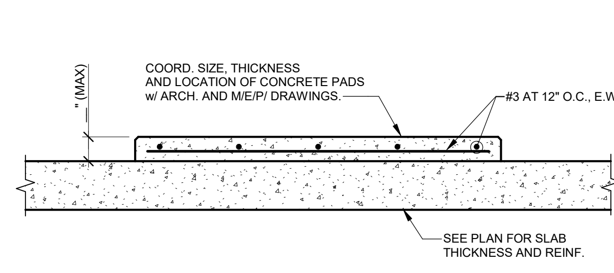
TYPICAL HOUSEKEEPING PAD (FOR M/E/P EQUIPMENT)
