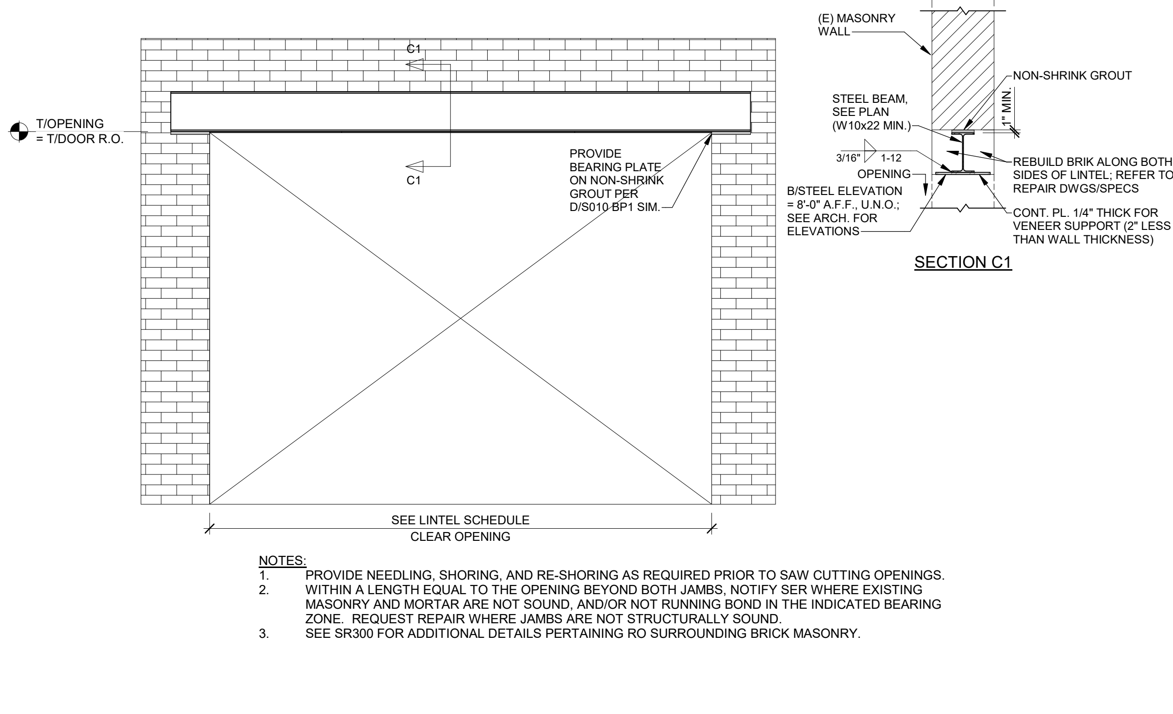
NEW DOOR/WINDOW OPENING IN EXISTING BRICK WALL - WIDE FLANGE LINTEL
