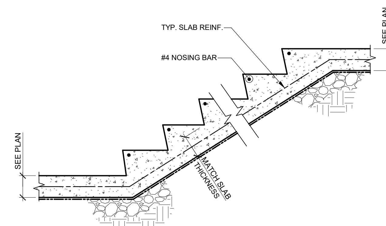
TYPICAL INTERIOR STAIR-ON-GRADE
