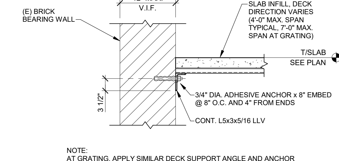
TYPICAL FLOOR SUPPORT AT EXISTING BRICK WALL
