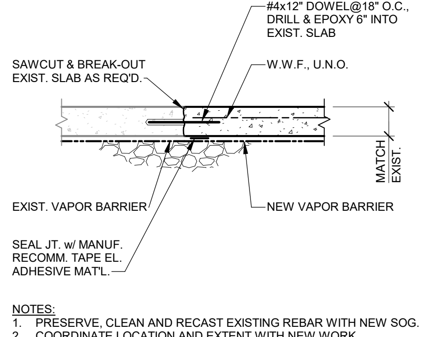
TYPICAL SLAB-ON-GRADE REPAIR
