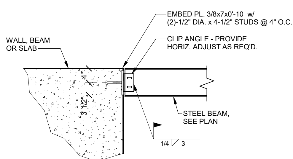
TYPICAL ELEVATOR DIVIDER BEAM CONNECTION
