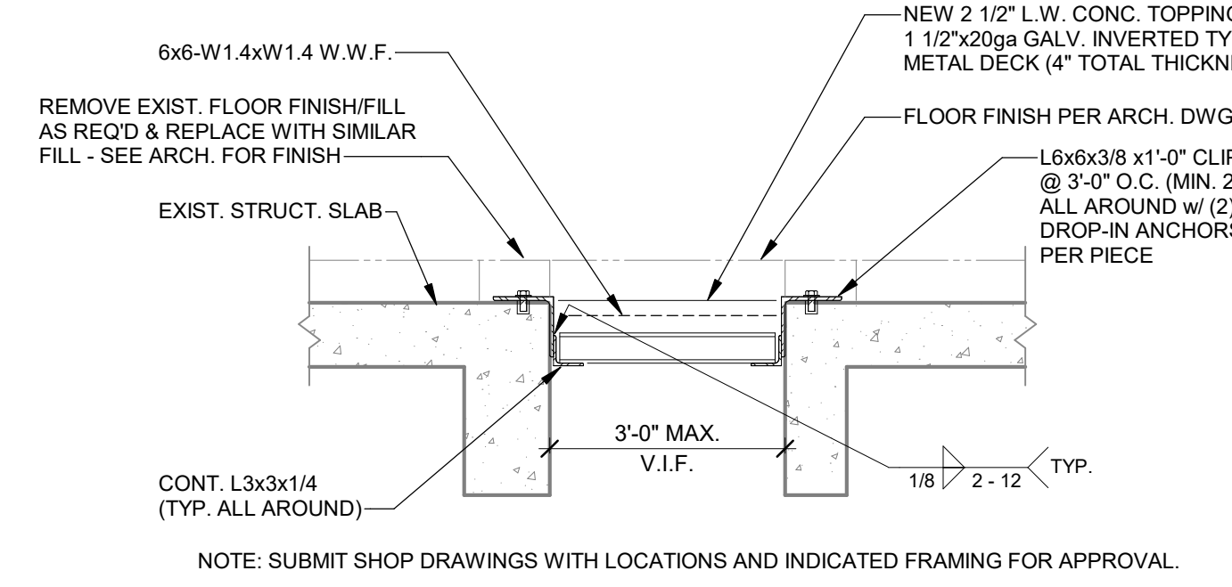
TYPICAL EXISTNG SLAB INFILL DETAIL
