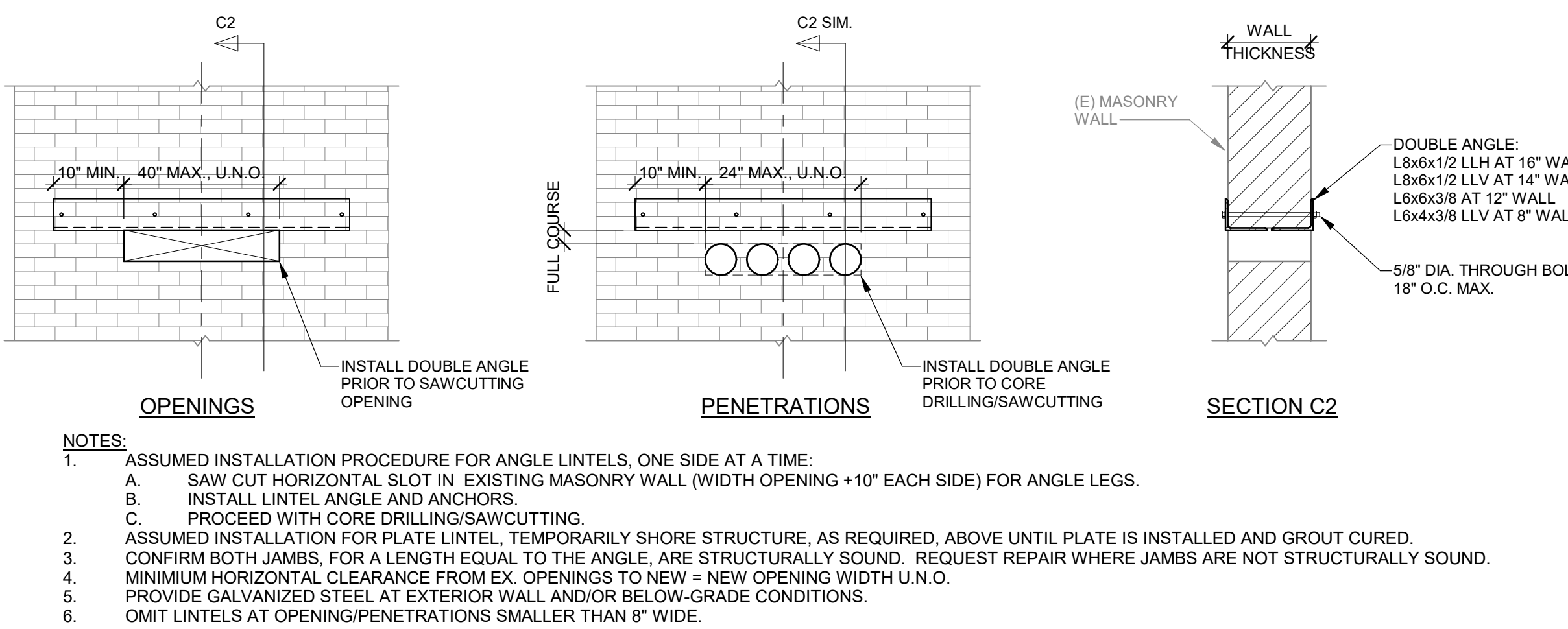
NEW MECHANICAL OPENINGS AND PENETRATIONS IN EX. BRICK WALL
