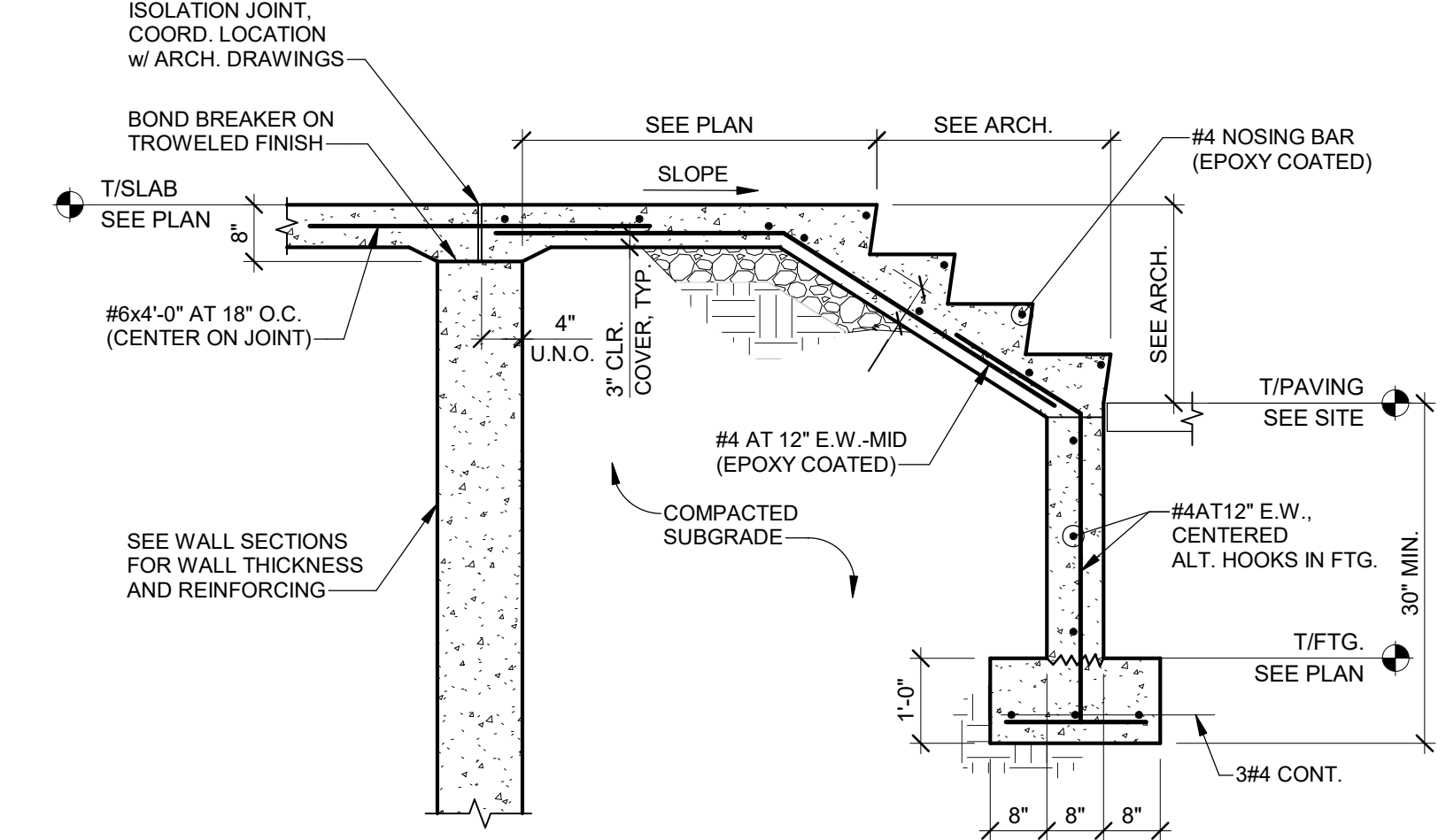
TYPICAL EXTERIOR STAIR
