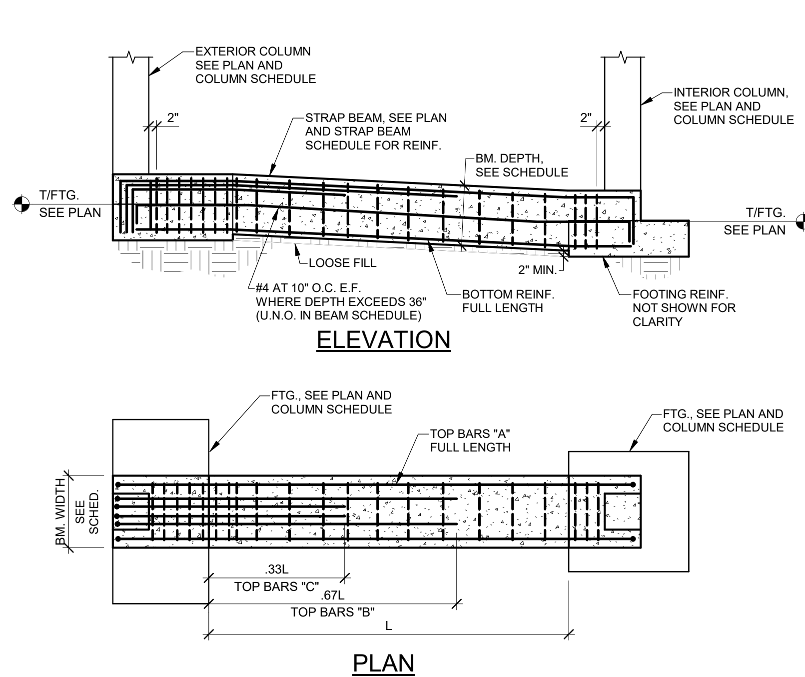
TYPICAL STRAP BEAM DETAIL
