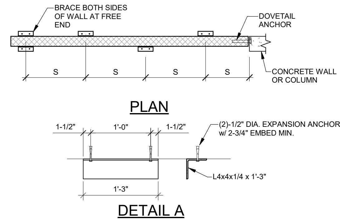
DETAIL A
