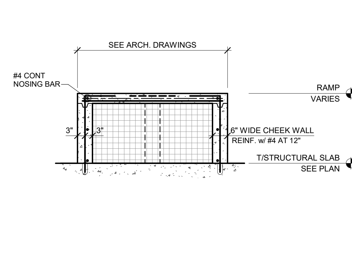
SECTION 1
