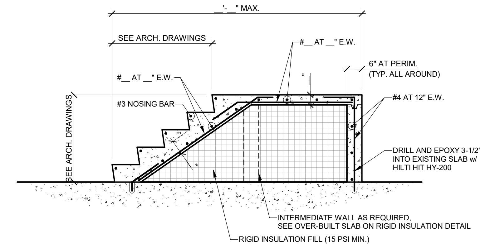
TYPICAL OVER-BUILT SLAB
