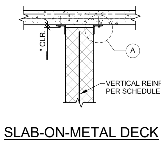
SLAB-ON-METAL DECK
